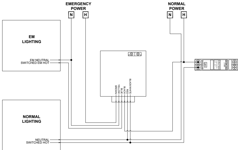
UL924 WIRING DETAIL (ESRN-1)
